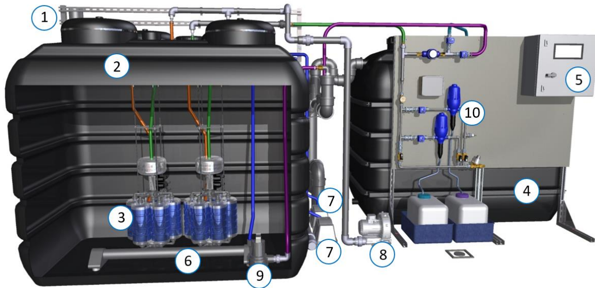
Figure 1: Overview: Packaged system AQUALOOP Greywater Recycling System 10800 l/day
