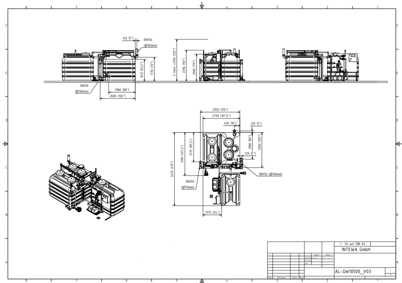
Figure 2: Dimensions and connections AQUALOOP AL-GW10800 I/d
